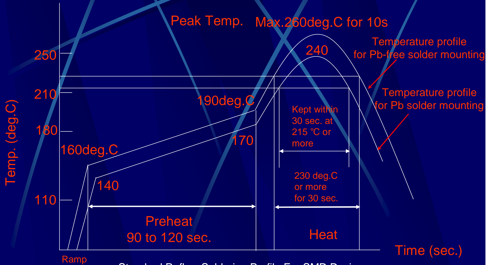
Standard Reflow Soldering Profile For SMD Devices
